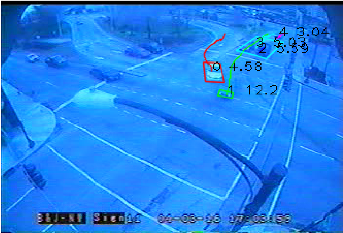
Motion Prediction
