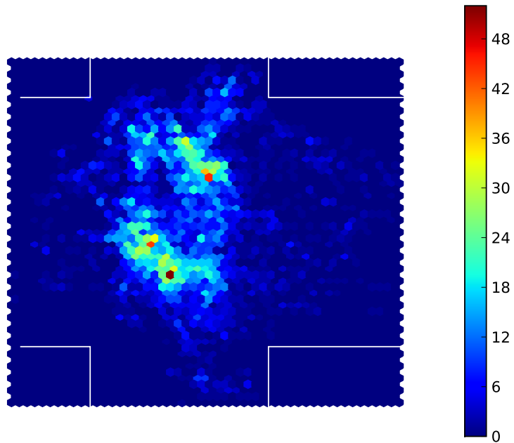
Collisions
