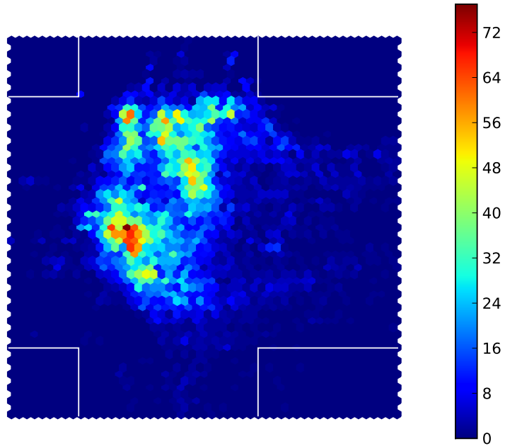
Traffic Conflicts
